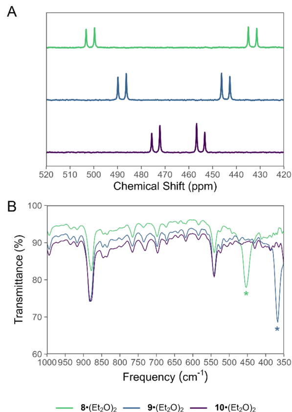
Fig. 3 Stacked (A) ^{31}\text{P} NMR spectra and (B) IR spectra of 8 ·(Et 2 O) 2 , 9 ·(Et 2 O) 2 , and 10 ·(Et 2 O) 2 . Signals in the IR spectrum assigned to a P–X bond stretching mode are denoted with an asterisk.
