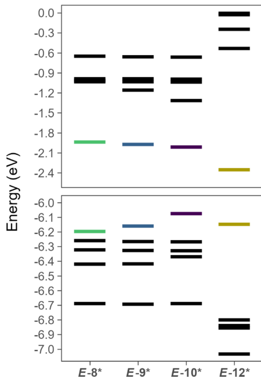
Fig. 7 Calculated orbital energies (DKH-PBE0/old-DKH-TZVPP//PBE0/def2-TZVPP) for E -8*, E -9*, E -10*, and E -12* with frontier molecular orbitals shown in color. The upper panel contains the values for the LUMO, LUMO+1, LUMO+2, LUMO+3, and LUMO+4. The lower panel contains values for the HOMO, HOMO-1, HOMO-2, HOMO-3, and HOMO-4.
