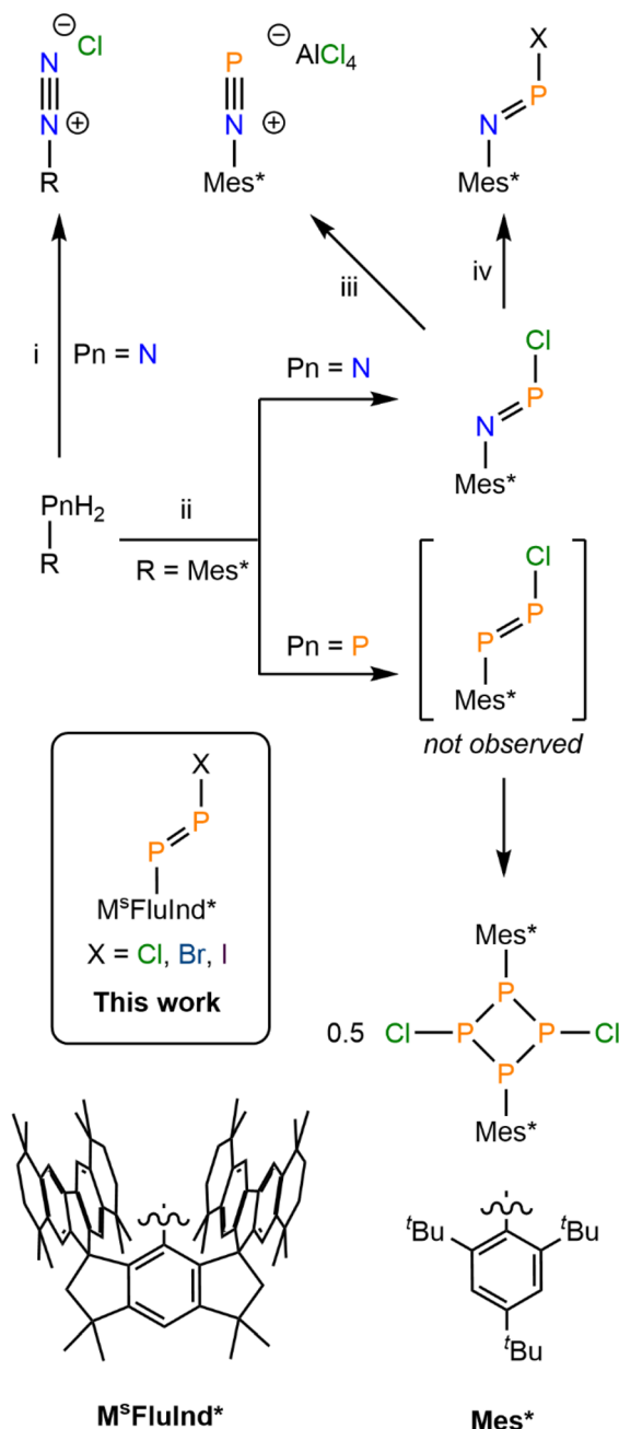
Fig. 1 General synthesis of [RNN][Cl] (i = excess HCl, excess NaNO 2 ). Synthesis of (Mes*)N=PCl and [ClP(μ-PMes*)] 2 (ii = excess PCl 3 , excess Et 3 N). Synthesis of [(Mes*)NP][AlCl 4 ] (iii = AlCl 3 ). Synthesis of (Mes*)NPX (iv = TMSX; X = Br, I). Depiction of (M s FluInd*)PPX (X = Cl, Br, I) reported herein. Structural diagrams of ligands M s FluInd* and Mes*.
