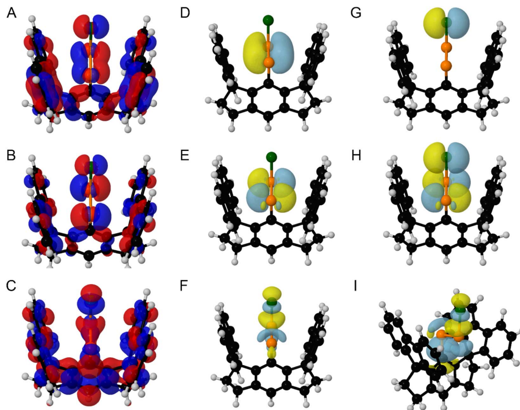
Fig. 6 (A) HOMO, (B) LUMO, and (C) LUMO+2 of E -8* (isovalue = 0.015). Surface plots (isovalue = 0.06) for E -8*, depicting the (D) P–P \pi bonding NLMO, (E) P–P \pi^* antibonding NLMO, (F) P–Cl \sigma^* antibonding NLMO, (G) a Cl-centered lone pair, (H) overlap between a Cl-centered lone pair and the P–P \pi^* antibonding NLMO, and (I) overlap between the P–C \sigma bonding NLMO and the P–Cl \sigma^* antibonding NLMO. In Fig. 6A–H, the molecule is viewed down the plane defined by the {PPCl} unit. In Fig. 6I, the molecule is oriented differently for clarity of the displayed NLMOs. Color code: P orange, Cl dark green, C black, H grey. Displayed NLMOs are pre-orthogonalized. Calculations were performed at the (DKH-PBE0/old-DKH-TZVPP//PBE0-D3/TZVPP) level of theory.
