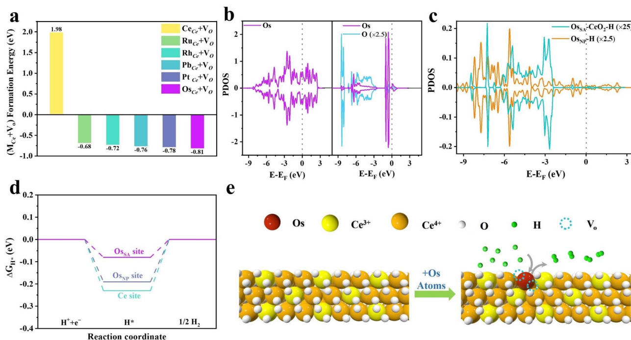
Fig. 1 Theoretical calculations illustrating the strong interfacial coupling of Os SAs in \text{CeO}_2 . (a) Calculated formation energies of M_{\text{Ce}} + \text{V}_{\text{O}} (M stands for the substituted atom for Ce). PDOS for (b) Os 5d orbital of \text{Os}_{\text{NP}} (left) and \text{Os}_{\text{SA}}\text{-CeO}_2 (right) and (c) H 1s orbital of adsorbed H. (d) Gibbs free energy diagram for the HER in acid media on \text{Os}_{\text{NP}} (blue line) and \text{Os}_{\text{SA}}\text{-CeO}_2 (purple and cyan lines). (e) Schematic mechanism of proton adsorption on the Os site leading to \text{H}_2 generation.
