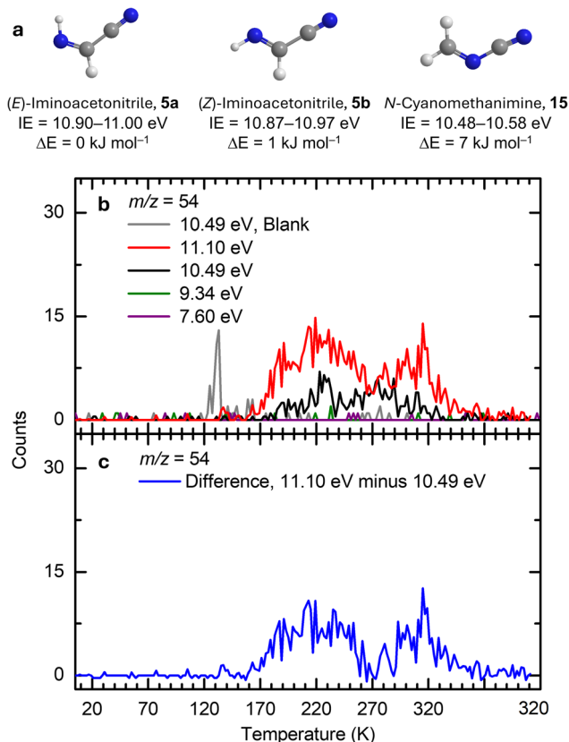
Fig. 5 Ion signals of hydrogen cyanide (1) ices during TPD at m/z = 54 . (a) Computed IEs and relative energies of \text{C}_2\text{H}_2\text{N}_2 isomers calculated at the CCSD(T)/CBS//B3LYP/aug-cc-pVTZ level of theory. (b) TPD profiles recorded at photon energies of 11.10, 10.49, 9.34, and 7.60 eV. TPD profiles of m/z = 54 were each recorded twice at 11.10 eV and 10.49 eV and the difference in their averaged profiles (c).
