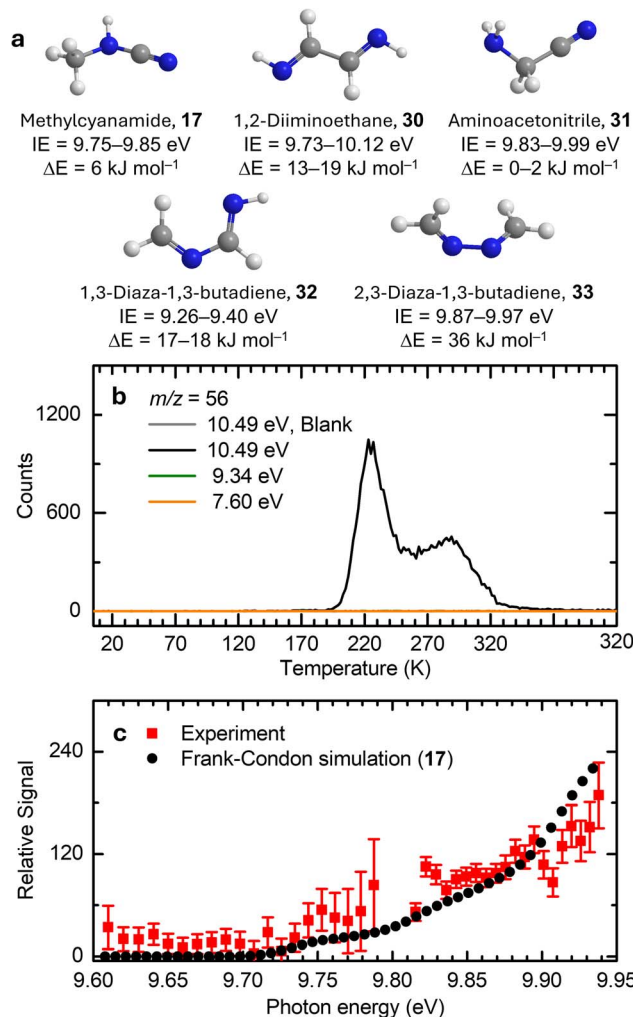
Fig. 6 Ion signals of hydrogen cyanide (1) ices during TPD at m/z = 56 and photoionization efficiency (PIE) curves. (a) Computed IEs and relative energies of \text{C}_2\text{H}_4\text{N}_2 isomers calculated at the CCSD(T)/CBS//B3LYP/aug-cc-pVTZ level of theory. (b) TPD profiles recorded at photon energies of 10.49, 9.34, and 7.60 eV. (c) PIE curve plotted as a function of photon energy after correcting for the TPD profile measured from 281 to 320 K. The Franck–Condon simulation of the PIE curve of methyl cyanamide ( 17 , black dots) is scaled for comparison with the experimental results.
