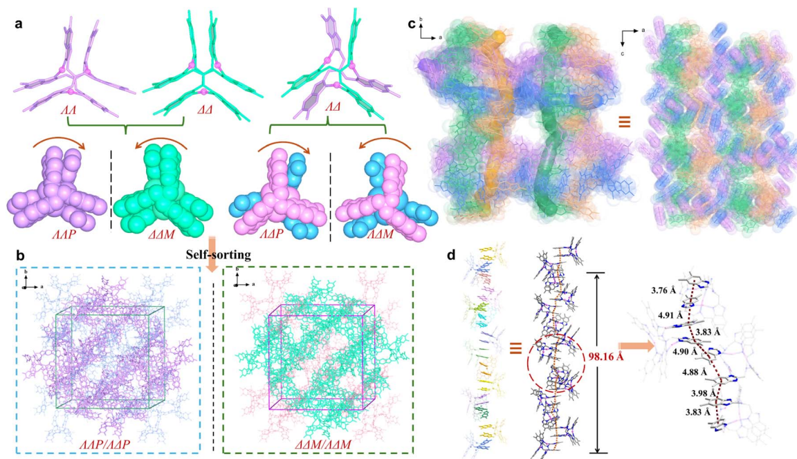
Fig. 2 Crystal structure of 3a . (a) \Delta\Delta P -, \Delta\Delta M -, \Delta\Delta P -, and \Delta\Delta M - [\text{Ag}_3\text{L}_3]^{3+} in 3a-P or 3a-M . (b) Narcissistic self-sorting of [\text{Ag}_3\text{L}_3]^{3+} forming chiral structures of 3a-P and 3a-M . (c) One of the channels along the c axis constructed by quadruple helices in 3a-P . (d) One of the \pi -stacked helical columns with a pitch of \sim 98.16 Å.
