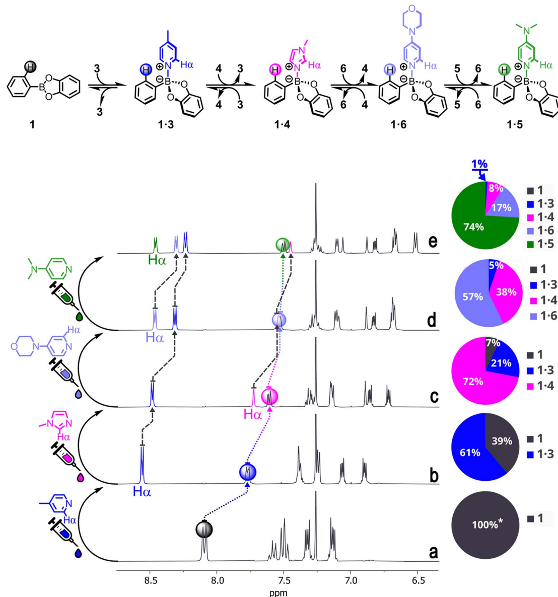
Fig. 5 Top: Simplified reaction scheme for the consecutive generation of DLs containing compounds 1 (black), 3 (blue), 4 (pink), 6 (light purple), and 5 (green), in order of addition) together with complexes 1·3, 1·4, 1·6, and 1·5 (in order of increasing stability). Bottom: NMR spectra of 1 (trace a); a mixture of 1 and 3 (trace b); a mixture of 1, 3, and 4 (trace c); a mixture of 1, 3, 4, and 6 (trace d); a mixture of 1, 3, 4, 6, and 5 (trace e). In each spectrum, the signal relative to each H \alpha proton is highlighted in the same colour as the NArHet (see structures). The H ortho proton is marked with a circle in the colour corresponding to the most prevalent adduct. To the right of each spectrum, a pie chart reports the calculated speciation of each DL. See Tables S17 and S18 for the ChemEQL-assisted speciation of the mixtures. All compounds are added 12.5 mM in CDCl 3 , the spectra are recorded at 25 °C. Only the aromatics region is shown. See Fig. S53 for the full spectra. * = in the absence of any ligands, 1 is in equilibrium with a small amount (<5% in our conditions) of phenylboronic acid and catechol due to partial hydrolysis from traces of water in the solvent. The addition of NArHets suppresses this side-reaction.
