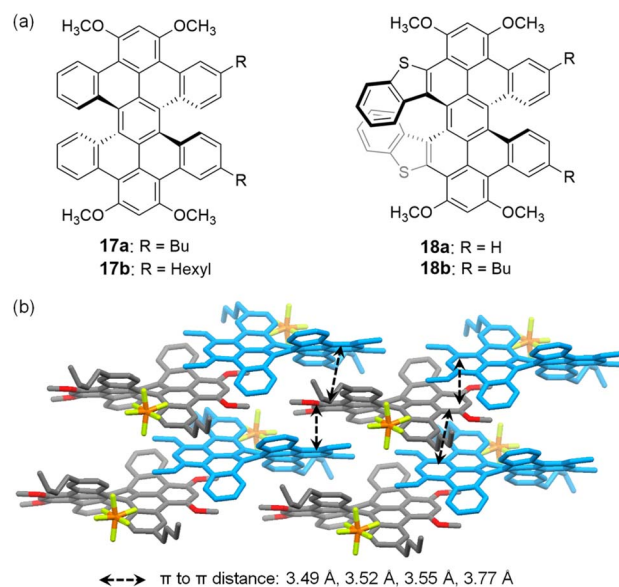
Fig. 6 (a) Double helicenes 17a/b and 18a/b ; (b) \pi – \pi stacking in the crystal of \text{17a}^{\bullet+}\text{PF}_6^- , where the (M, M) enantiomer is shown in blue, and the (P, P) enantiomer is colored according to the elements. Reproduced with permission from ref. 40. Copyright 2022 American Chemical Society.
