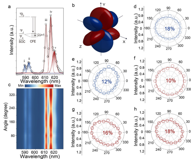
Fig. 4 Polarization properties of the Eu-NC. (a) Spectral fitting of the {}^5\text{D}_0 \rightarrow {}^7\text{F}_1 (MDT) and {}^5\text{D}_0 \rightarrow {}^7\text{F}_2 (EDT) transitions was performed using the 0^\circ polarized emission spectrum. The peaks and their corresponding area integrals are assigned distinct colors. Inset: spin–orbit coupling (SOC) and crystal field effect (CFE). (b) Orientation of magnetic transition dipoles and rotors of \text{Eu}^{3+} ions in a single crystal of the Eu-NC. (c) Angle-dependent polarized PL spectra of Eu-NC microrods (ca. 0 – 360^\circ ). (d–h) Angle-dependent photoemission intensities of the Eu-NC microrods of the selected areas. d–h correspond to the degrees of polarization at peaks i–v in (a): 589, 593, 611, 615, and 620 nm, respectively.
