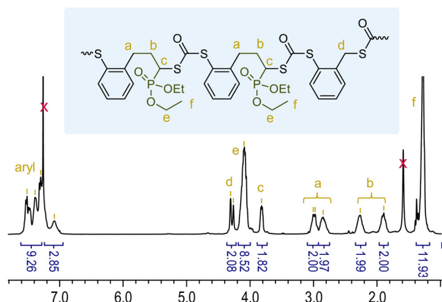
Fig. 5 ^1\text{H} NMR spectrum of \text{p}(\text{DEVP}_{0.4}\text{-BOT}_{0.6})_n (Table 1, entry 8).
