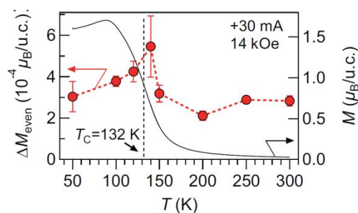
Figure 6. Temperature dependency of the current induced magnetization (red dots). The solid black line shows the magnetic susceptibility of bulk crystal without current.
