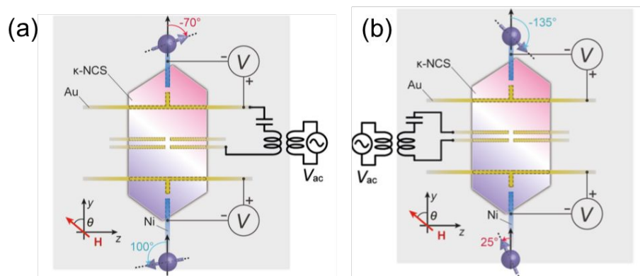
Figure 8: Schematic diagram of the non-local spin measurement with a Janus-type crystal composed of a right-handed domain (red area) and a left-handed domain (light blue area). (a) The right-handed domain was excited by AC and the outward spin pair was detected. (b) The left-handed domain was excited by AC and the inward spin pair was observed. The opposite spin directions observed at opposite edges indicate a \mathcal{T} -odd spin configuration, corresponding to CISS(II).
