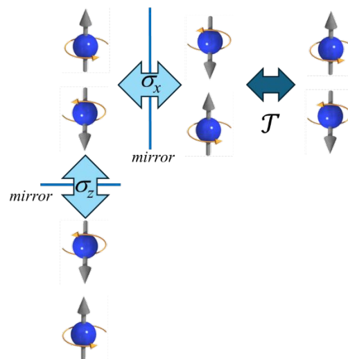
Figure 3: Conceptual diagram of antiparallel spin pairs. Mirror operations on the x - or z -direction with respect to outward antiparallel spin pairs result in inward antiparallel spin pairs, which are not superimposable with the original structure. Importantly, this conversion between enantiomers can also be achieved by time-reversal operations \mathcal{T} .
