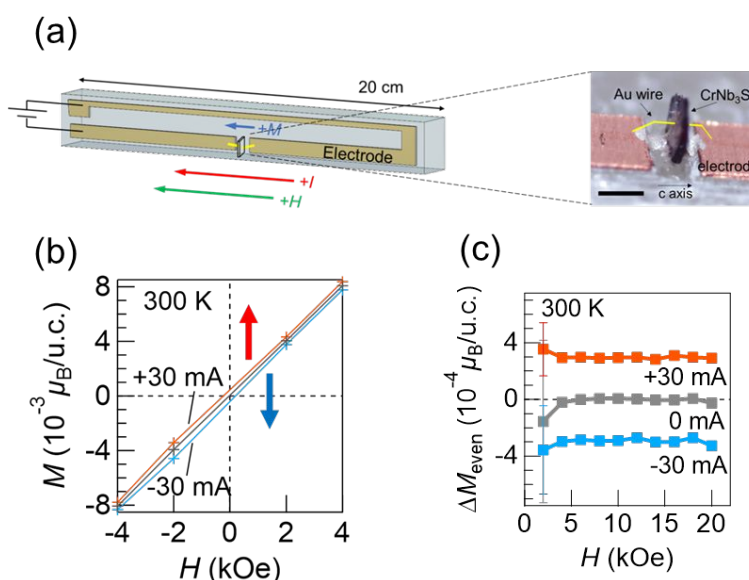
Figure 5. (a) Experimental setup for SQUID measurement under applied current. The stray Oersted field was kept small by elongated electrode configuration. (b) Magnetization curve with and without applied current. (c) Current induced magnetization measured in various magnetic field.
