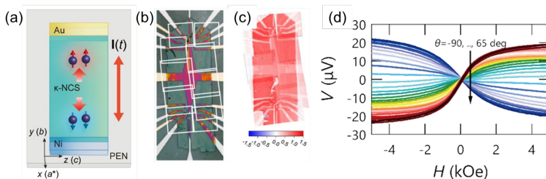
Figure 7: (a) Schematic of the CISS experiment with \kappa -NCS. AC bias was applied in the b axis direction to drive the spin rectification. (b) Microscopic image of the device. White squares show CD microscope fields of view. (c) CD microscope image of the crystal which shows right-handed structure in the entire crystal. The field of view is identical to Fig. 1b. (d) Angle dependent voltage V across the nickel and gold electrodes. Magnetization M of the nickel electrode was rotated by the external
