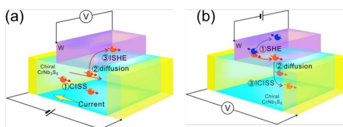
Figure 4. Schematic diagram of spintronics device composed of \text{CrNb}_3\text{S}_6 and tungsten (W) electrode. In CISS mode (a), a bias current was applied to \text{CrNb}_3\text{S}_6 and the polarized spin diffused into W to generate transverse voltage by ISHE. On the other hand, in iCISS mode (b), a spin polarization was created by SHE in W and diffused into \text{CrNb}_3\text{S}_6 to induce voltaic effect by iCISS. The observed spin signal satisfies Onsager reciprocity and corresponds to a \mathcal{T} -even response, consistent with CISS(I). The output voltage was linear to the input current in both cases.
