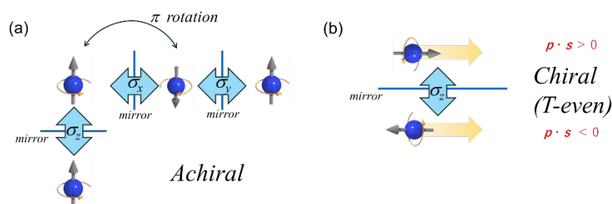
Figure 2: Electron spin and chirality. (a) The spin of a localized electron reverses under a mirror operation parallel to the spin, but returns to the original state upon 180^\circ rotation. (b) Electrons with spin polarization collinear with momentum reverse the sign of helicity under a mirror operation and never return to the original state, no matter how much they rotate.
