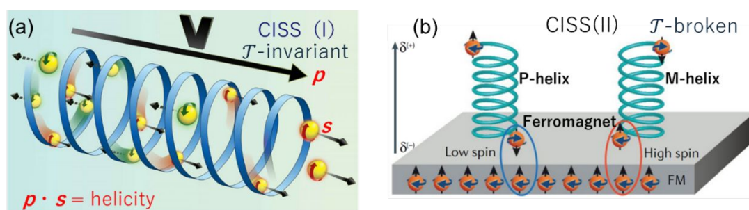
Figure 1: The conceptual image for (a) CISS(I) and (b) CISS(II). After time-reversal ( \mathcal{T} ), the system remains the same in CISS(I), but the situation becomes opposite for CISS(II): in the right panel, P-helix has outward spin pair that forms singlet-spins with ferromagnetic substrate. This outward spins on P-helix will become inward spins and up-spin in the substrate will become down-spin after time-reversal. Then, down-spin polarized substrate will also have singlet-exchange interaction with the P-helix, which contradicts with experiment. Therefore, \mathcal{T} is broken in the right panel. Note that ferromagnetic substrate is used only for detecting the \mathcal{T} -breaking of the chiral molecule, so that \mathcal{T} -breaking of the substrate is not essential in this discussion. Figure 1(a) is adapted from ref 1c with permission from ACS, copyright 2016. Figure 1(b) is adapted from ref 6 with permission from AAAS, copyright 2018.
