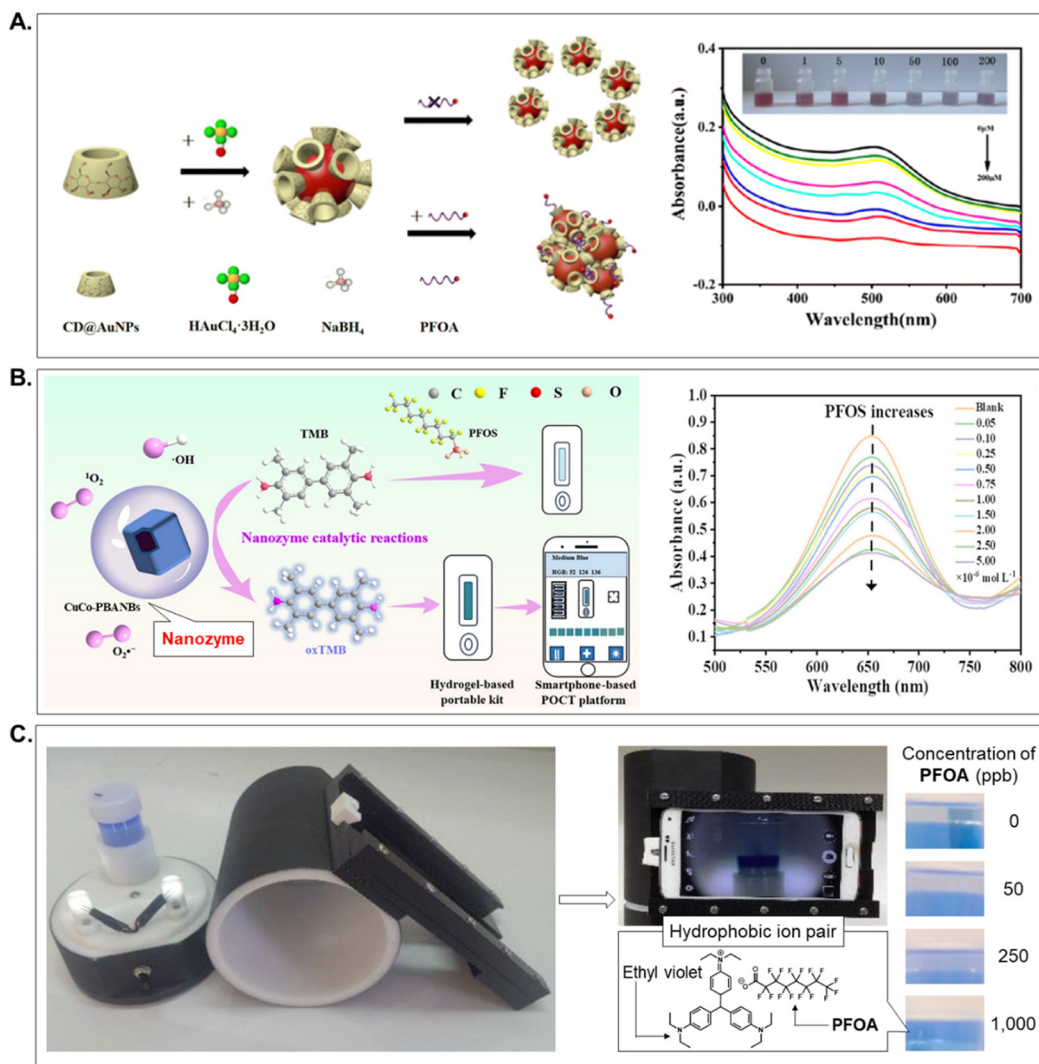
Fig. 3 Schematic of the colorimetric detection mechanism of specific PFASs: (A) aggregation induced by specific PFAS adsorption on Au NP surfaces; (B) inhibition of colouration resulting from specific PFAS adsorption onto the surface of nanozymes catalysing ROS generation; (C) monitoring the colour change of a solution containing hydrophobic ion pairs formed by dyes and specific PFASs using askCARE™. Reproduced with permission from ref. 63, Copyright 2025 Royal Society of Chemistry; ref. 65, Copyright 2024 American Chemical Society; and ref. 80 Copyright 2018 Elsevier.
