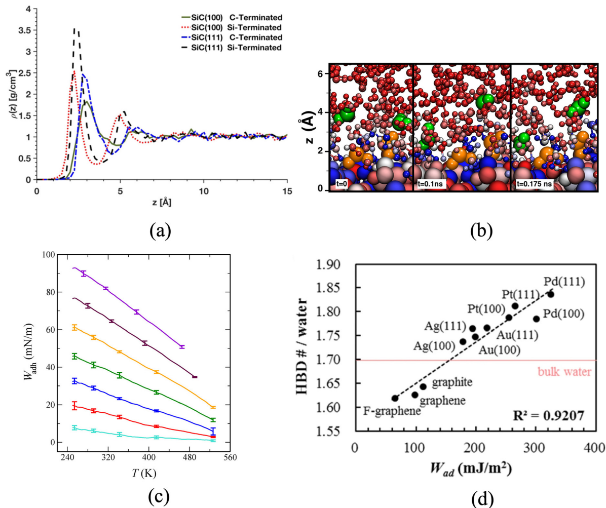
Fig. 10 (a) Interfacial water density profiles perpendicular to 3C-SiC surfaces with different crystallographic planes and atomic terminations. Si-terminated surfaces exhibit higher first-layer adsorption peaks and more extended liquid layering compared to C-terminated surfaces, reflecting stronger solid-liquid interactions and enhanced hydrophilicity. Reproduced with permission from ref. 87. Copyright 2018 American Chemical Society. (b) Molecular dynamics snapshots of interfacial water at an amorphous alumina-water interface. Atoms are colored by instantaneous heat transfer rate (red: low, white: medium, blue: high). Tracked water molecules in deep potential wells (orange) remain spatially confined with restricted mobility, while those in weaker interaction regions (green) retain greater translational and rotational freedom. Adapted with permission from ref. 87. Copyright 2021 American Chemical Society. (c) Temperature dependence of the work of adhesion W_{\text{ad}} for water near a Lennard-Jones 9-3 wall at varying substrate strengths. Curves from bottom to top correspond to surface strengths of \epsilon_{\text{sf}} = 0.831, 1.66, 2.49, 3.33, 4.16, 4.99 , and 5.82 \text{ kJ mol}^{-1} . Adapted with permission from ref. 213. Copyright 2013 American Chemical Society. (d) Number of hydrogen-bond donors (HBDs) per water molecule in the adlayer region as a function of surface hydrophilicity, quantified by the work of adhesion ( W_{\text{ad}} ). Data span hydrophobic carbon surfaces (fluorographene, graphene, graphite) to hydrophilic metal surfaces (Ag, Au, Pt, Pd) with (100) and (111) facets. The horizontal dashed line indicates the bulk water value of 1.70. The strong linear correlation ( R^2 = 0.92 ) demonstrates that hydrogen-bond network connectivity serves as a molecular-level descriptor of macroscopic wettability. Reproduced from ref. 63, under the terms of the Creative Commons Attribution 4.0 License (CC BY 4.0). Changes: none.
