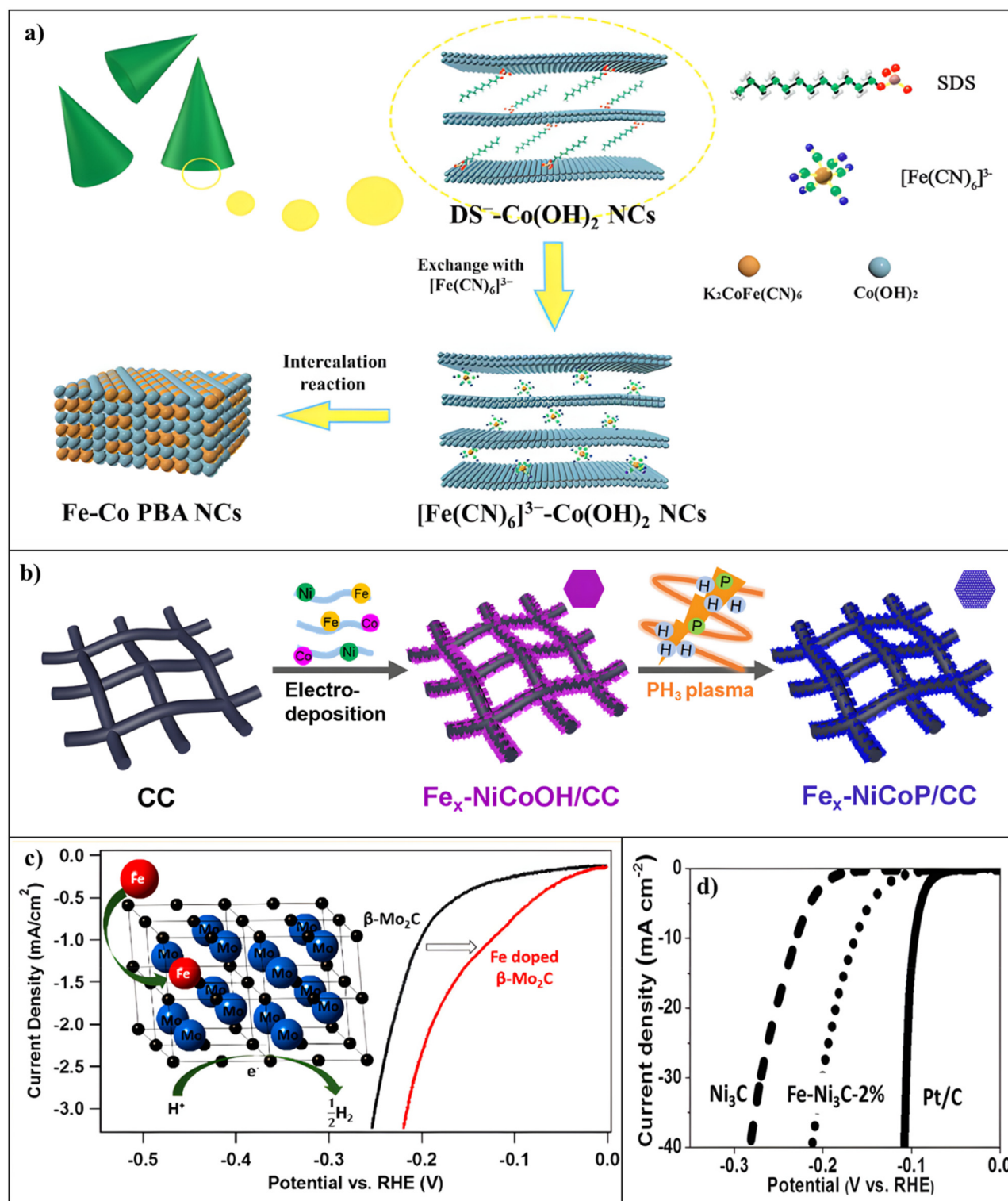
Fig. 6 (a) Schematic illustrating the mechanism by which Fe-Co PBA NCs emerges from Co(OH) 2 NCs. Reproduced from ref. 61 with permission. Copyright 2018, ACS. (b) A diagrammatic illustration of the Fe x -NiCoP/CC synthesis method. Reproduced from ref. 62 with permission. Copyright 2020, ACS. (c) Polarisation curves for Fe-doped β-Mo 2 C and pure β-Mo 2 C. Reproduced from ref. 66 with permission. Copyright 2015, ACS. (d) Sample polarisation curves for Ni 3 C, Fe-Ni 3 C-2%, and Pt/C in 0.5 M H 2 SO 4 . Reproduced from ref. 70 with permission. Copyright 2017, Wiley.
