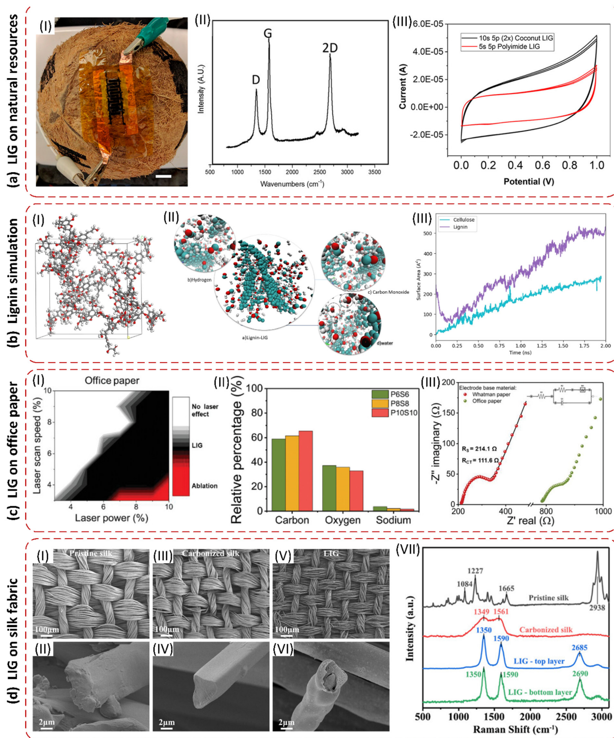
Fig. 8 Bio-based material for LIG. (a) LIG grown on lignin-rich natural solids. (I) LIG-based supercapacitor fabricated on coconut. (II) Raman spectrum of coconut-derived LIG laser twice (10% speed and 5% power). (III) CV curves of a twice-lased coconut micro-supercapacitor compared with a single-lased polyimide at a scan rate of 10 \text{ mV s}^{-1} . This figure has been adapted from ref. 33 with permission from American Chemical Society, copyright 2018. (b) Simulation of LIG on lignin. (I) Lignin simulation box. (II) Visualization of simulation and gasses evolved during the process. (III) Calculated surface area of LIG from lignin and cellulose. This figure has been adapted from ref. 118 with permission from Springer Nature, copyright 2024. (c) LIG grown on paper. (I) Heat maps of the laser irradiation effect on office paper. (II) Relative element composition of LIG on office paper. (III) Nyquist plots of chromatography paper and office paper to interpret EIS data. This figure has been adapted from ref. 124 with permission from John Wiley and Sons, copyright 2021. (d) LIG grown on silk fabric. (I) SEM image of the fabric structure of pristine silk. (II) SEM image of a single fiber of pristine silk. (III) SEM image of the fabric structure of carbonized silk. (IV) SEM image of a single fiber of carbonized silk. (V) SEM image of the fabric structure of LIG. (VI) SEM image of a single fiber of LIG. (VII) Raman spectra of pristine silk, carbonized silk, and LIG. This figure has been adapted from ref. 131 with permission from John Wiley and Sons, copyright 2021.
