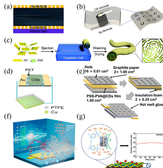
Fig. 4 (a) Cross-sectional diagram of CDs/paper device. 25 Reproduced from ref. 25 with permission from Royal Society of Chemistry, copyright 2018. (b) Preparation process of the MEG device based on PA-CPDs. 83 Reproduced from ref. 83 with permission from John Wiley and Sons, copyright 2023. (c) Schematics showing the wet-spinning process of the GQD-GO fiber. 42 Reproduced from ref. 42 with permission from Royal Society of Chemistry, copyright 2019. (d) Humidity sensors based on carbon nanodots. 84 Reproduced from ref. 84 with permission from Elsevier, copyright 2022. (e) Schematic illustration of the fabrication process for a MEG. 85 Reproduced from ref. 85 with permission from Elsevier, copyright 2023. (f) Working principle of the GQD moisture triggered nanogenerator. 12 Reproduced from ref. 12 with permission from American Chemical Society, copyright 2017. (g) Moisture electricity generation performance and hydrogen bond network structure of PPG-MEG. 43 Reproduced from ref. 43 with permission from American Chemical Society, copyright 2024.
