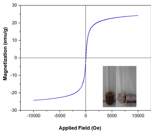
Fig. 6 VSM diagram of Mag@RF/SB-Cu.
