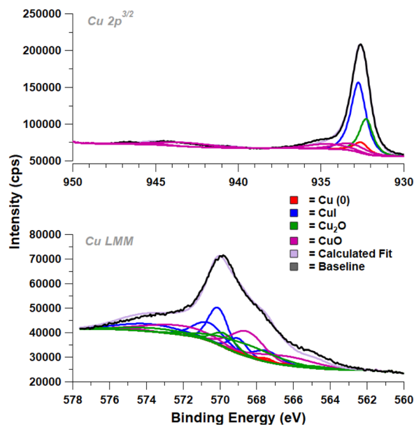
Fig. 5 XPS spectra of the clean region of vial 1 and associated fits from copper surface species.
