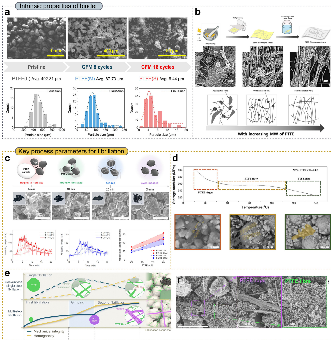
Fig. 4 (a) SEM images (top) and particle size distribution (bottom) of cryo-pulverized PTFE powders. Reproduced with permission from ref. 76. Copyright 2024, Elsevier B.V. (b) Processing schematic of the solid electrolyte sheet formation (top). SEM image (middle) and a predictive fibrillation model for different molecular weights (bottom). Reproduced with permission from ref. 85. Copyright 2024, Elsevier B.V. (c) Schematic illustration of the morphological changes of the PTFE binder with kneading time (top), corresponding SEM images (middle), and kneading torque profiles (bottom). Reproduced with permission from ref. 55. Copyright 2024, Elsevier B.V. (d) Storage modulus of PTFE at different temperatures (top) and corresponding SEM images (bottom). Reproduced with permission from ref. 77. Copyright 2024, Wiley-VCH GmbH. (e) Schematic illustration of the multi-step fibrillation process (left) and SEM images of rope- and fiber-like PTFE morphologies at different feeding times (right). Reproduced with permission from ref. 88. Copyright 2025, The Royal Society of Chemistry.
