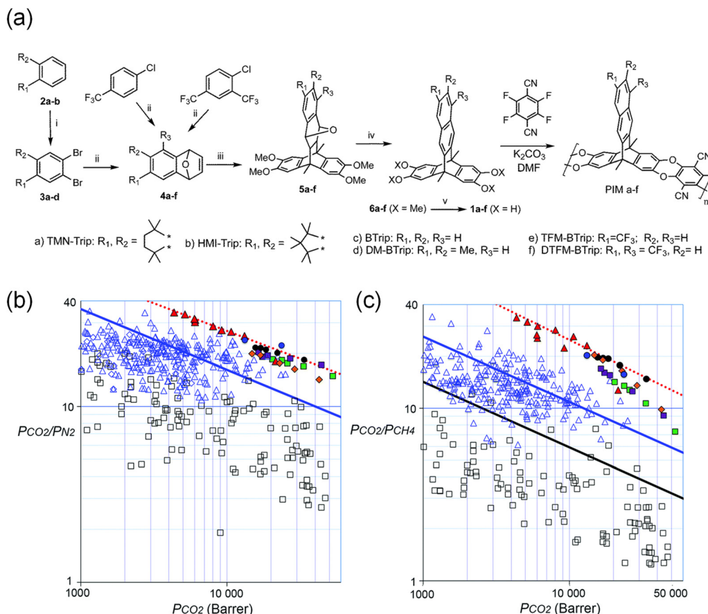
Fig. 11 (a) Structure and synthetic route of benzotriptycene-based PIMs. Reaction conditions: (i) \text{Br}_2 , Fe, DCM, rt, 3 h; (ii) n\text{-BuLi} , furan, THF, -78^\circ\text{C} , 1.5 h; (iii) 9,10-dimethyl-2,3,6,7-tetramethoxyanthracene, DMF, 250^\circ\text{C} , 7 bar, microwave irradiation, 2 h; (iv) TFA or \text{MeSO}_3\text{H} , rt, 24 h; (v) \text{BBr}_3 , DCM. (b) and (c) Robeson plots for (b) \text{CO}_2/\text{N}_2 and (c) \text{CO}_2/\text{CH}_4 separation, showing the gas-permeability performance of benzotriptycene-based PIM films. The proposed revised upper bounds for both gas pairs are indicated by red dashed lines. 15
