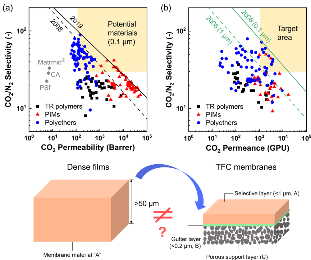
Fig. 21 Proposed knowledge gap between intrinsic material performance ( i.e. , permeability) and practical membrane performance ( i.e. , permeance). (a) Literature survey of \text{CO}_2 permeability (unit: Barrer) measured from dense films of TR polymers, PIMs, and polyether-based polymers. 14,15,23,38,81 The black dashed and solid lines represent the 2008 14 and 2019 15 upper bounds for polymeric membranes for \text{CO}_2/\text{N}_2 separation, respectively. The yellow box indicates candidate materials that could reach the target performance for post-combustion capture when coated as a 0.1 \mu\text{m} -thick selective layer. 13 (b) Literature survey of gas permeance (unit: GPU) measured from TFC membranes. 23,38,101 The green dashed line denotes the separation performance upper bound for a 1 \mu\text{m} -thick selective layer derived from the 2008 upper bound, 14 while the green solid line denotes the corresponding upper bound for a 0.1 \mu\text{m} -thick selective layer. The yellow box indicates the target \text{CO}_2/\text{N}_2 separation performance for post-combustion capture. 13 Most separation performances were measured at temperatures ranging from 25 to 35 ^\circ\text{C} and pressures from 1 to 2 bar, including both pure-gas and mixed-gas \text{CO}_2/\text{N}_2 separation data. Of note, facilitated transport membranes are also important candidates for \text{CO}_2 separation; however, they are excluded here because standardized benchmarks for a fair comparison with solution-diffusion-mechanism-based polymer membranes are not yet established. All data presented herein are sourced from ref. 101.
