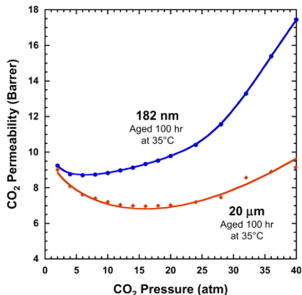
Fig. 22 CO 2 plasticization pressure profiles for thin (182 nm) and thick (20 μm) Matrimid® films prepared with identical thermal histories. 70 Reproduced from ref. 70 with permission from Elsevier, copyright 2011.
