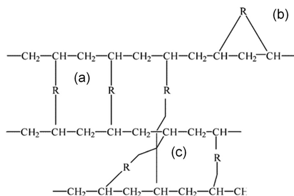
Fig. 16 Schematic representation of typical network elements in XLPEGDA. PEGDA features the repeating unit \text{CH}_2\text{CH}(\text{R})\text{CH}_2\text{CH}_2 . (a) The smallest possible network segment; (b) a wasted cross-link or loop; (c) an entanglement that becomes permanent due to cross-linking. 88 Reproduced from ref. 88 with permission from American Chemical Society, copyright 2005.
