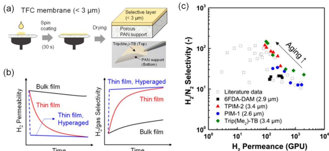
Fig. 23 (a) Schematic representation of the fabrication process for PIM-based thin-film composite (TFC) membranes. (b) Illustration of how physical aging influences H 2 separation in PIMs, comparing bulk films, thin films, and hyperaged thin films. (c) Comparison of H 2 /N 2 separation performance for PIM-based TFC membranes with values reported in the literature. Arrows indicate the evolution of gas-separation properties over 0–336 h. 107 Reproduced from ref. 107 with permission from Elsevier, copyright 2023.
