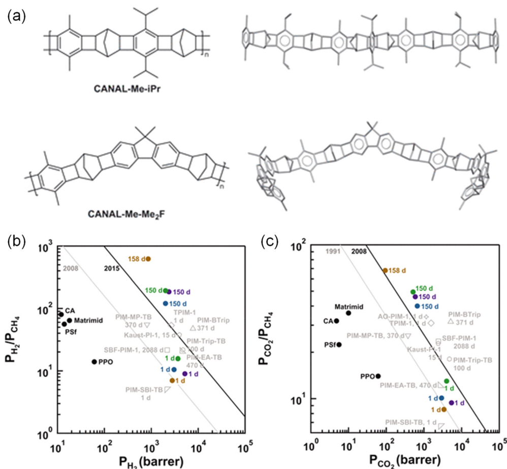
Fig. 13 (a) (Left) Experimental and (right) molecular-mechanics–simulated structures of a ribbonlike 2D ladder polymer (CANAL-Me-iPr, top) and a 3D ladder polymer (CANAL-Me-Me 2 F, bottom). Me = methyl; iPr = isopropyl. (b) and (c) Pure-gas permeation data for 50–60 μm thick films of CANAL-Me-Me 2 F (purple), CANAL-Me-S5F (green), CANAL-Me-S6F (blue), and CANAL-Me-DHP (brown), plotted relative to the (b) H 2 /CH 4 and (c) CO 2 /CH 4 upper bounds. 69 Reproduced from ref. 69 with permission from The American Association for the Advancement of Science, copyright 2022.
