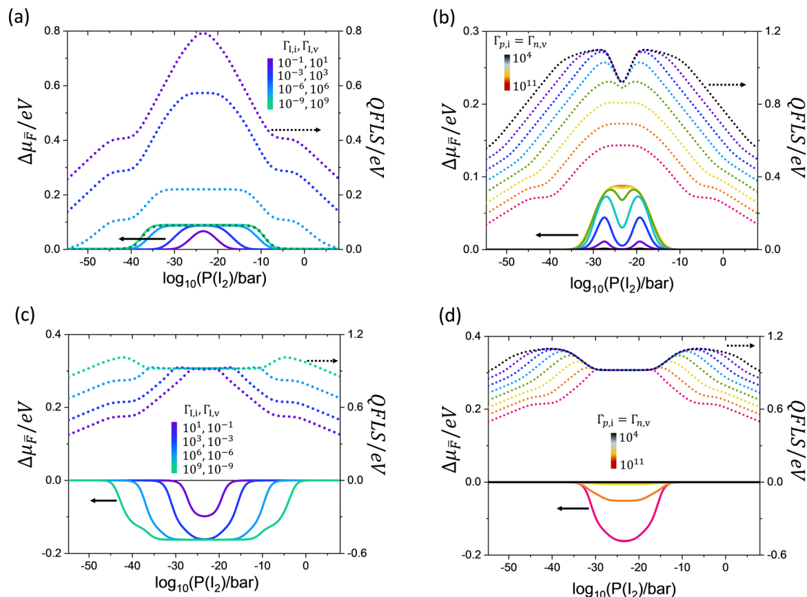
Fig. 8 Dependence of the ionic ( \Delta\mu_{\text{F}} ) and electronic (QFSL) change in chemical potential on the \Gamma_{\text{li}} , \Gamma_{\text{lv}} , and \Gamma_{\text{pi}} , \Gamma_{\text{nv}} parameters, as a function of P(l_2) . Trends for (a) increasing h_{\text{ion}} > 0 ( \Gamma_{\text{pi}} = \Gamma_{\text{nv}} = 10^{11} ), (b) increasing \Gamma_{\text{pi}} = \Gamma_{\text{nv}} ( \Gamma_{\text{li}} = 10^{-3} , \Gamma_{\text{lv}} = 10^3 ), (c) decreasing h_{\text{ion}} < 0 ( \Gamma_{\text{pi}} = \Gamma_{\text{nv}} = 10^{11} ), and (d) increasing \Gamma_{\text{pi}} = \Gamma_{\text{nv}} ( \Gamma_{\text{li}} = 10^3 , \Gamma_{\text{lv}} = 10^{-3} ). All remaining parameters are the same as the ones used in Fig. 3. h_{\text{ion}} = \log_{10}\left(\frac{\Gamma_{\text{lv}}}{\Gamma_{\text{li}}}\right) .
