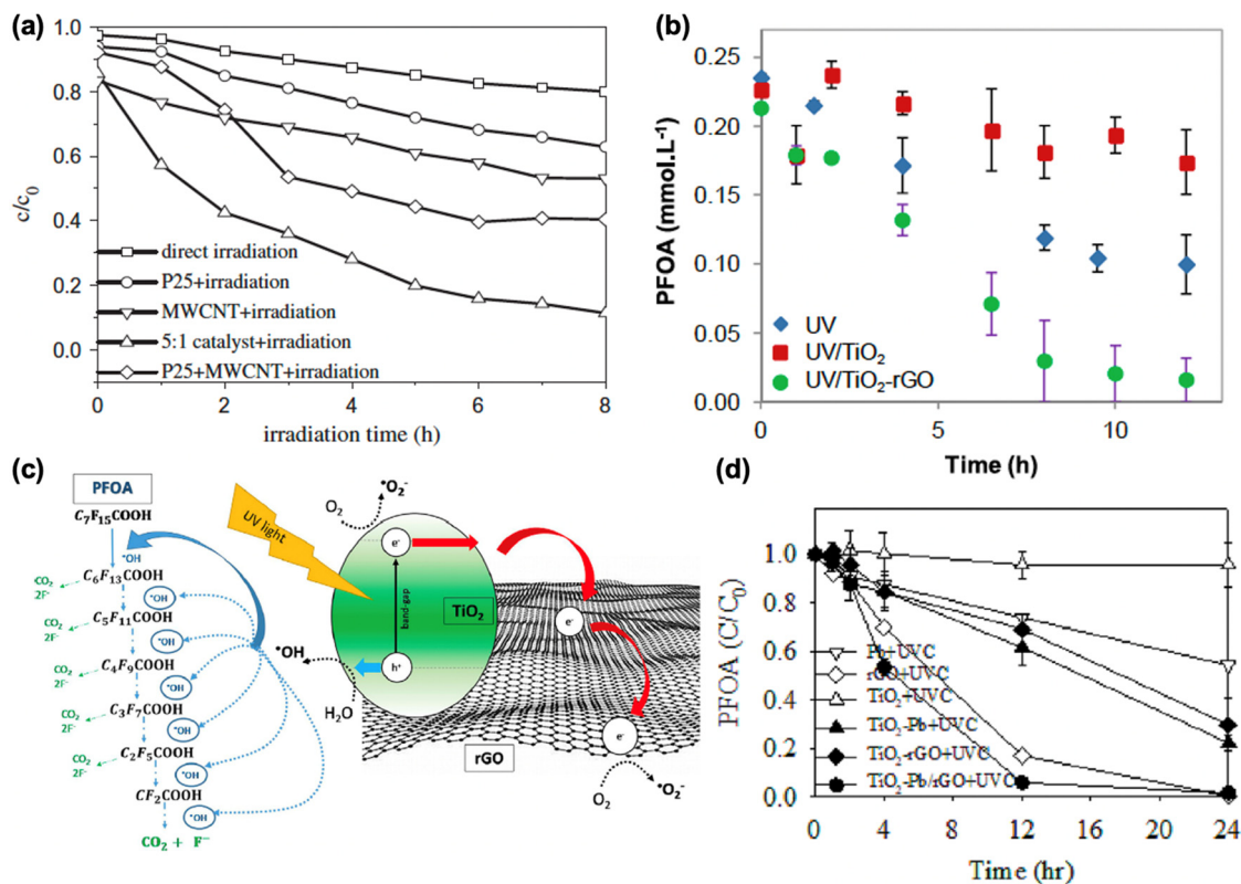
Fig. 12 Photocatalytic degradation of PFOA and PFOS over various \text{TiO}_2 -based and modified photocatalysts: (a) comparison with a physical mixture of P25 and MWCNTs (5:1). Reproduced from ref. 265 with permission from Elsevier BV, copyright 2012; 265 (b) comparison of PFOA degradation after 12 h under UV irradiation using \text{TiO}_2 , \text{TiO}_2 -rGO composite, and GO control, showing enhanced removal with \text{TiO}_2 -rGO due to improved light penetration and reduced electron-hole recombination, (c) proposed photocatalytic degradation pathway of PFOA over \text{TiO}_2 -rGO, highlighting the role of rGO in enhancing charge separation, radical generation ( \cdot\text{OH} and \text{O}_2^{\cdot-} ), stepwise perfluoroalkyl cleavage, and eventual formation of \text{CO}_2 and \text{F}^- . reproduced from ref. 266 with permission from Elsevier BV, copyright 2018; 266 (d) PFOA removal under UVC irradiation using \text{TiO}_2 , Pb, rGO, \text{TiO}_2 -Pb, \text{TiO}_2 /rGO, and \text{TiO}_2 -Pb/rGO, showing enhanced degradation with composite materials due to synergistic effects of rGO and Pb doping. Reproduced from ref. 267 with permission from Wiley, copyright 2023.
