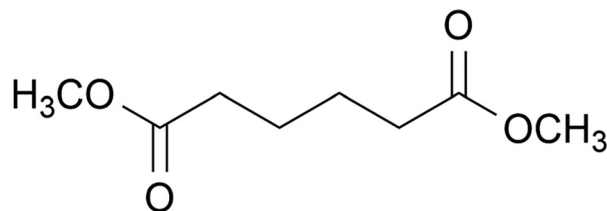
Fig. 1 (A) A general chemical formula of phthalate ester plasticizer, and (B) the non-phthalate ester plasticizer (DMA).
