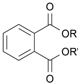
Fig. 1 (A) A general chemical formula of phthalate ester plasticizer, and (B) the non-phthalate ester plasticizer (DMA).
