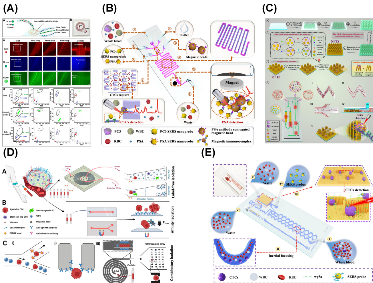
Fig. 3 (A). Separation effect of fluorescent microspheres by inertial microfluidic chip. Separation diagram of mixture of three types of micro-particles with diameter of 5 μm, 10 μm and 20 μm (A); photograph of inertial microfluidic chip with inlet, spiral channel, and outlets (B), fluorescent pictures of particles' trajectories in inlet, first loop, third loop, fifth loop and outlets (C), comparison of fluorescent intensity and proportion of particles in collected liquid sample from inlet, central outlet and both side outlets (D). 38 (B). Schematic of simultaneous separation and SERS detections of CTCs and PSA in an integrated microfluidic chip. 129 (C). (a) Schematic illustration of the NFTS fabrication process. (b) Sequential process for preparing two different types of antibody-conjugated SERS nanotags; (c) Schematic illustration of the modification of capture aptamers on NFTS and subsequent CTCs capture process. (d) The workflow of multistage capture and in situ single-cell phenotype analysis with SERS measurement for PCa CTCs on CMD. 130 (D). Microfluidic CTC isolation technologies. (A) Label-free, (B) affinity-based, and (C) combinatory isolation. 132 (E). Schematic diagram of CTCs captures and SERS detections on microfluidic chip. 133 Reproduced from ref. 38, 129, 130, 132 and 133 with permission from Royal Society of Chemistry, Elsevier, Elsevier, American Chemical Society, and Elsevier, respectively; copyright 2024, 2025, 2025, 2024, and 2025.
