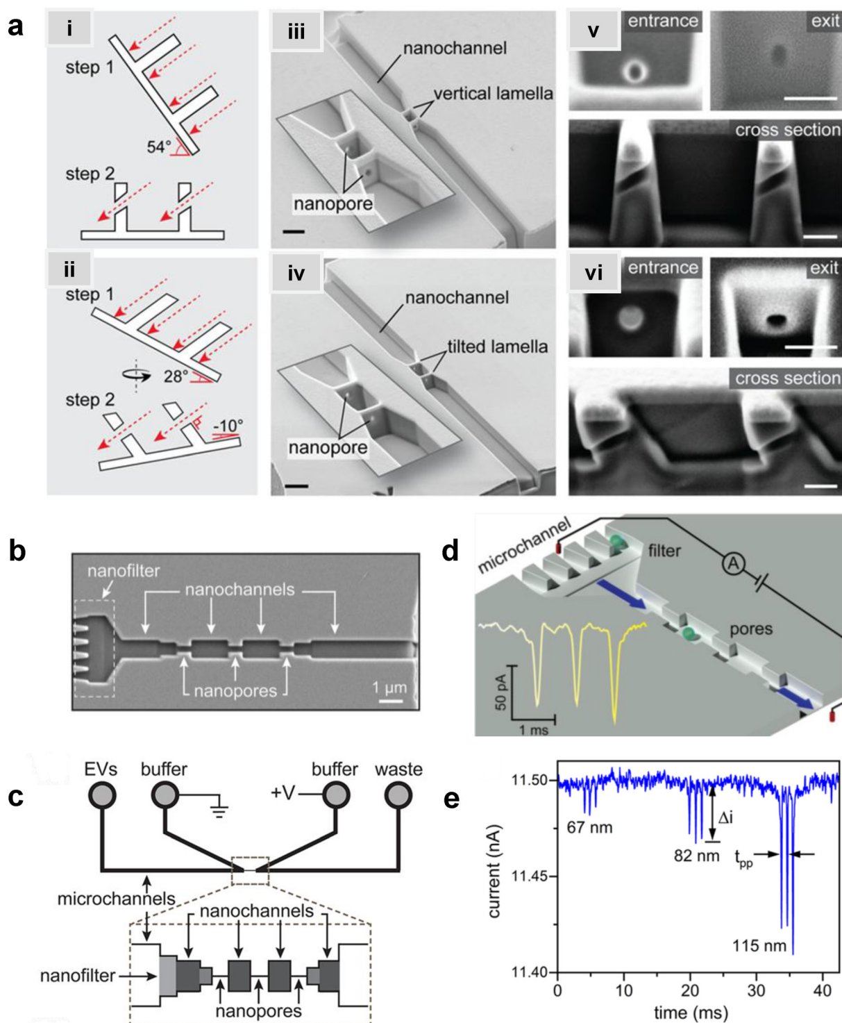
Fig. 7 Glass in-plane nanopore devices. (a) Schematic view of vertical (i) and tilted lamella (ii) fabricated by adjusting the stage and the incident beams angles (iii), SEM images of vertical lamella (iii) and tilted lamella (iv) holding two in-plane circular nanopores directly milled on the lamella walls (scale bar: 1 μm). SEM images of conical (v) and cylindrical (vi) nanopore shapes initiated due to lamella wall alignments (scale bar: 200 nm). Reproduced from Zhang et al. 85 with permission from American Chemical Society. (b) SEM image of three in-plane nanopores milled by FIB instrument. (c) Schematic diagram of the entire device containing 4 reservoirs, 2 V-shape microchannels, nanofilters, nanochannels and nanopores. (d) A visual illustration of the EV particles translocating through the nanopores and generating current transient amplitudes. (e) Current transient amplitudes of 67, 82 and 115 nm EV particles. Reproduced from Young et al. 23 with permission from American Chemical Society.
