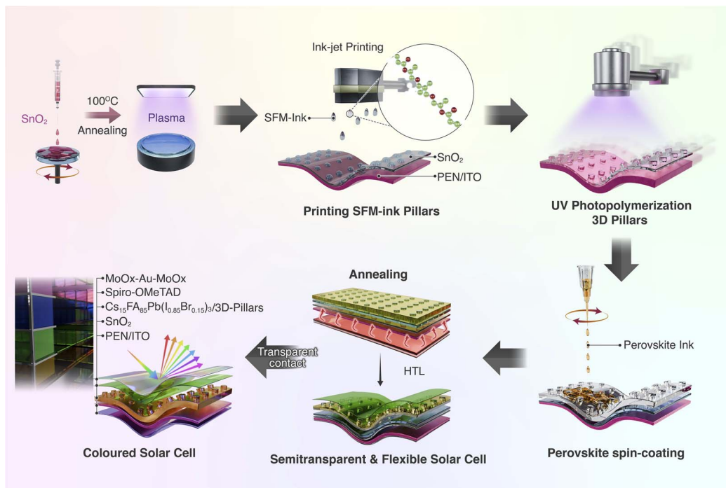
Fig. 1 Schematic presentation of the main steps involved in the fabrication of a colourfull, semi-transparent, flexible perovskite solar cell.
