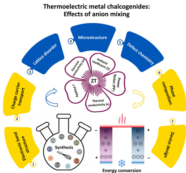
Fig. 1 Positive effects of anion mixing in metal chalcogenide thermoelectrics: (1) tailoring band gap, band alignment, and band convergence; (2.1) balancing charge carrier effective mass, concentration, and mobility; (2.2) controlling conductivity type; (2.3) suppressing bipolar effects; (3) introducing mass fluctuation and local strains; (4) designing hierarchical heterogeneity; (5) adjusting formation energies and solubility limits; (6.1) synthesizing favorable secondary phases; (6.2) stabilizing favorable phases; (6.3) tailoring polymorphic transitions; (7.1) designing new flexible and wearable device architectures; (7.2) improving device thermomechanical stability.
