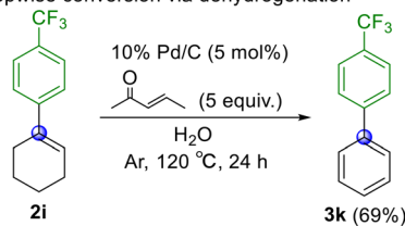
Fig. 5 One-pot biaryl synthesis from 1-arylcylohexanols: construction of benzene rings via Pd/C-catalyzed dehydration and dehydrogenation.
