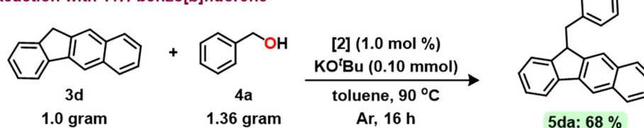
Fig. 2 Gram-scale synthesis.
