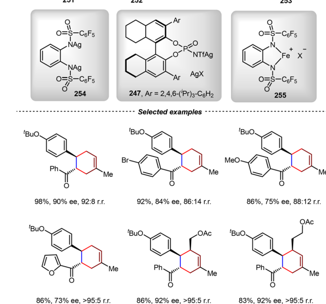
Scheme 51 A new \text{Fe}(\text{III}) photoredox catalyst consisting of a chiral phosphoramidate anion and an achiral bidentate ligand.
