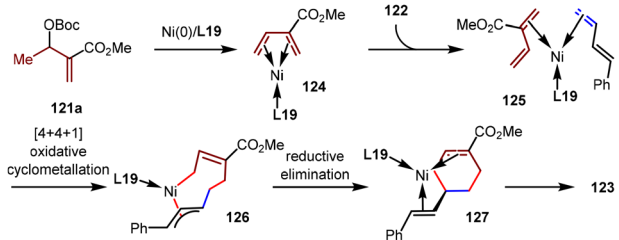
Scheme 28 Ni(0)-catalyzed [4+2] cycloadditions of Morita–Baylis–Hillman carbonates with 1,3-dienes.
