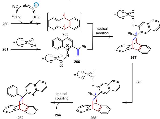
Scheme 53 Asymmetric [4+2] dearomative photocycloadditions of anthracene with alkenylazaarenes.
