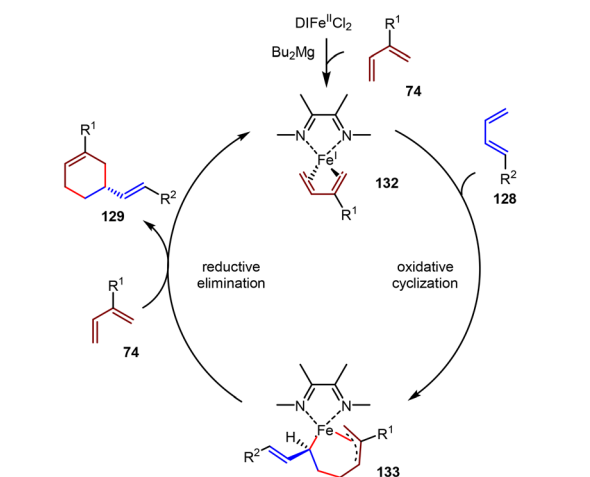
Scheme 29 Fe(II)/ \alpha -diimine-catalyzed asymmetric cross-[4+2] cycloadditions of unactivated 1,3-dienes.
