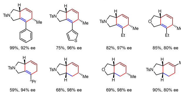
Scheme 31 \text{Co}(\text{I}) -catalyzed intramolecular [4+2] cycloaddition reactions of unactivated diene-yne and trienes.
