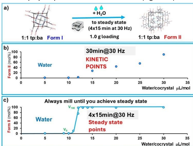
Figure 45 Effect of milling time on water steady-state solvent curves for 1:1 tp:ba cocrystals: (a) reaction scheme; (b) insufficient milling (30 minutes) yields scattered
