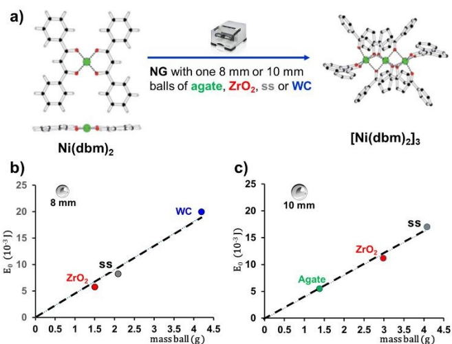
Figure 58 Mechanochemical trimerization of brown \text{Ni}(\text{dbm})_2 \rightarrow green [\text{Ni}(\text{dbm})_2]_3 . a) Reaction scheme. b, c) Activation impact energy ( E_0 ) as a function of milling ball mass ( m_{\text{ball}} ). b) 8 mm balls made from \text{ZrO}_2 , ss, and WC. c) 10 mm balls made from agate, \text{ZrO}_2 , and ss. The fraction of reactant powder affected by critical loading conditions per unit time ( k_{\text{cl}} ) correlates directly with E_0 . 74 Reproduced from ref. 74 with permission from [RSC], copyright [2022] and figures drawn with original data supplied by Maria Carta.
