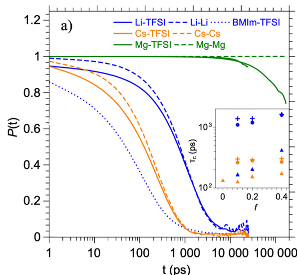
Fig. 6 Lifetime distribution of ion complexation and ion pairing/aggregation in [\text{X}][\text{BMImTFSI}]f electrolytes at T = 500 K. (a) Time correlation function P(t) of ion/ion solvent [BMIm-TFSI], alkali coordination [X-TFSI] and aggregation [X-X] for X = \text{Li}, \text{Cs} and \text{Mg} . Ion pairing corresponds to distances between ions which are shorter than the first minimum of the G(r) pair distributions. These distances are reported in Table S6. Inset: evolution of ion pairing time \tau_c as a function of the ratio f at T = 500 K. The symbols correspond to the (●) X-TFSI (+) X-X and (▲) BMIm-TFSI ion pair correlations.
