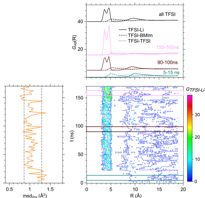
Fig. 8 Time dependence of the radial distribution function for a selected 'mean' TFSI in [Li][BMIm][TFSI]0.2 at T = 300 K. A sampling of 2 ns was selected to obtain statistically relevant dynamical, structural and cross-coupled information. Central view: 2D level map for G_{\text{TFSI-Li}}(r) . Top: projections of G_{\text{AB}}(r) for selected trajectory sections as underlined by the color rectangle on 2D map. Left: MSD calculated for a 2 ns range ( \text{MSD}_{2\text{ns}} ) along the trajectory. \text{msd}_{2\text{ns}} corresponding to "slow" and "fast" regime also presented as dashed lines.
