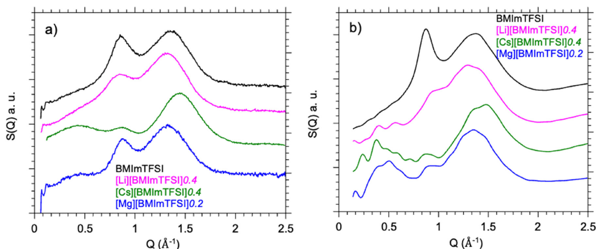
Fig. 2 WAXS diffraction pattern of pure BMImTFSI and [X][\text{BMImTFSI}]f electrolytes ( X = \text{Li}^+, \text{Cs}^+, f = 0.4 Mg 2+ f = 0.2 ) (a) experiments at room temperature (b) molecular dynamics at T = 300 K. These patterns are shifted vertically for the sake of clarity.
