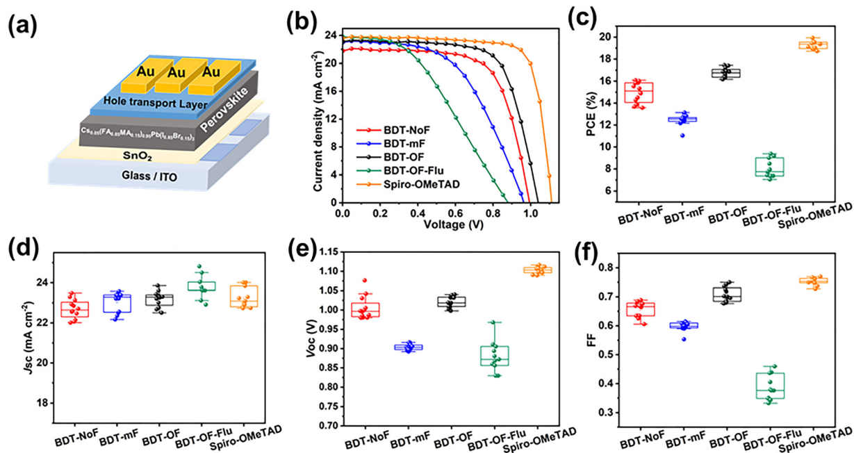
Fig. 5 (a) Schematic illustration of the PSC architecture incorporating HTMs. (b) Representative J-V curves of the devices measured under AM 1.5G illumination at 100 \text{ mW cm}^{-2} . (c)–(f) Statistical distributions of photovoltaic parameters for the PSCs (average of 12 cells for each architecture).
