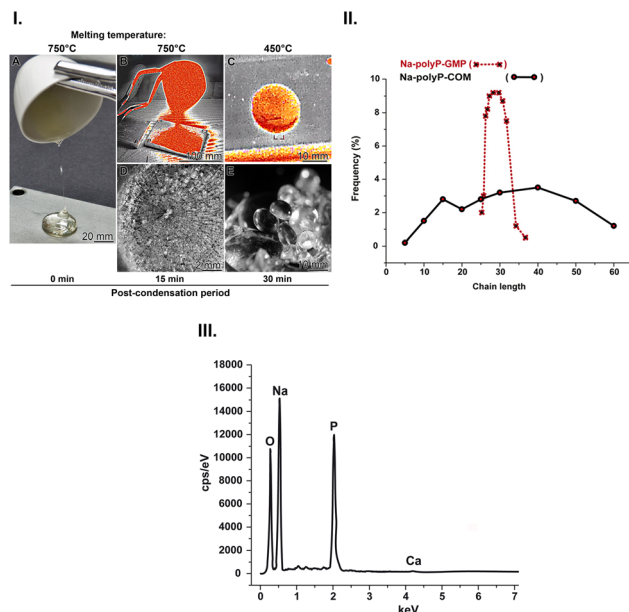
Fig. 1 Synthesis of Na-polyP from \text{NaH}_2\text{PO}_4 monomers. The polymer was prepared at 750 °C using a controlled polycondensation process, followed by accelerated cooling (B to C). (I.) (A) Pouring the melt from the crucible (83 mm upper diameter and 55 mm height). Two time points were chosen to demonstrate polyP lens formation; after a post-condensation period of (D) 15 min and (E) 30 min. Perfectly convex lenses are formed after 30 min. At time point 15 min, the lenses are still fused together. The images (B) and (C) were taken with an infrared camera; the square in (C) is the camera focus. (II.) The sharp distribution of polyP chain lengths (given in P_i units) of the Na-polyP-GMP polymer (red) in contrast to the broad size distribution of Na-polyP-COM (black). (III.) EDX spectrum for the Na-polyP-GMP formulation showed the prominent element peaks for Na, O, and P; the weak Ca peak originates from the crucible material.
