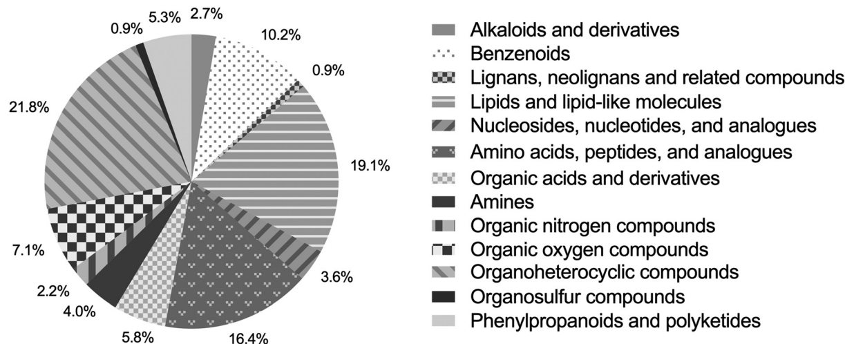
Fig. 2 Chemical classification of annotated metabolites. The pie chart illustrates the distribution of metabolites in the IPA control group (pH 8.2, n = 5 ). The proportions of chemical classes are labeled alongside each segment of the chart.
