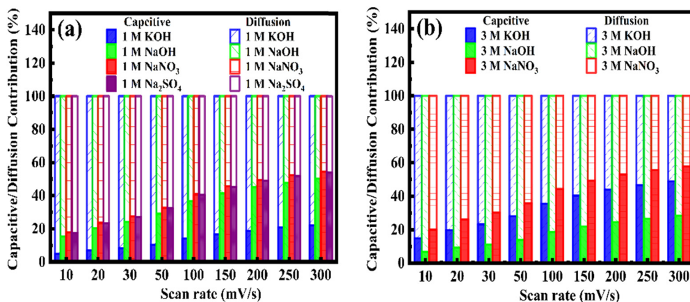
Fig. 12 Percentage capacitive and diffusion contribution to the total charge storage in the Mn 2 O 3 -9 mM urea sample measured in (a) 1 M and (b) 3 M electrolyte concentrations at different scan rates.
