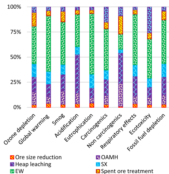
Fig. 2 The contribution of each stage to the whole process of producing one ton of copper.
