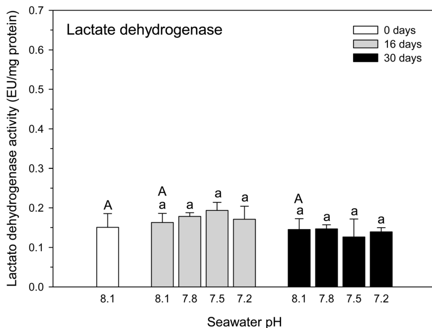
Fig. 3 Lactate dehydrogenase activity (UE per mg protein) in the hydrocoral Millepora alcicornis kept under the control condition (ambient seawater: pH 8.1) or exposed to different levels of CO 2 -driven seawater acidification (pH 7.8, 7.5 and 7.2) for 16 and 30 days in a marine mesocosm system. Data are expressed as mean \pm standard deviation ( n = 12 ). Different capital letters indicate significantly different mean values ( p < 0.05 ; one-way ANOVA, followed by the LSD test) under the control condition (pH 8.1) at the different experimental times (0, 16 and 30 days). Different lowercase letters indicate significantly different mean values ( p < 0.05 ; two-way ANOVA, followed by the LSD test) among the experimental conditions (exposure time and pH treatment).
