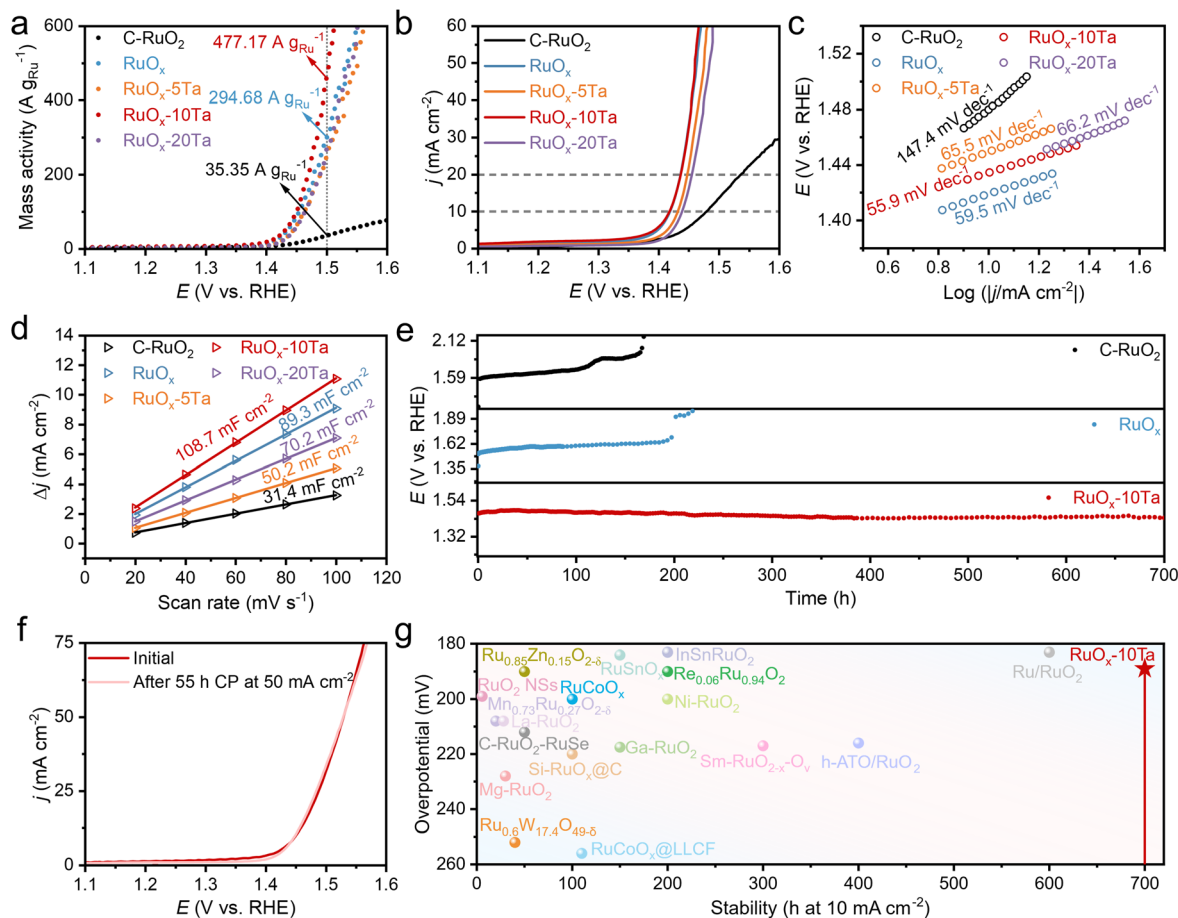
Fig. 2 Electrochemical performance. (a) LSV curves normalized by the Ru mass of \text{RuO}_x\text{-}\alpha\text{Ta} ( \alpha = 5, 10 and 20 ), homemade \text{RuO}_x and \text{C-RuO}_2 . (b) LSV curves of \text{RuO}_x\text{-}\alpha\text{Ta} , homemade \text{RuO}_x and \text{C-RuO}_2 . (c) Tafel plots derived from the polarization curves in (b). (d) Electrochemical double-layer capacitance ( C_{dl} ) of the electrocatalysts. (e) Chronopotentiometric plots of \text{C-RuO}_2 , \text{RuO}_x and \text{RuO}_x\text{-10Ta} at 10 \text{ mA cm}^{-2} . (f) LSV curves of \text{RuO}_x\text{-10Ta} before and after 55 h CP at 50 \text{ mA cm}^{-2} . (g) Comparison of the overpotential and durability of \text{RuO}_x\text{-10Ta} at j = 10 \text{ mA cm}^{-2} with those of the previously reported OER catalysts in acidic media.
