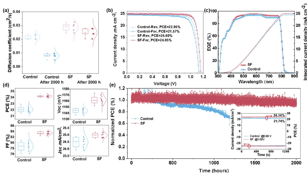
Fig. 5 (a) Statistical distribution of diffusion coefficients in perovskite films, extracted by fitting time-series carrier diffusion profiles from 20 sets of stroboscopic measurements. The data can represent the average carrier diffusion coefficient levels of the whole perovskite films: SF-treated and untreated films, both before and after 2000 hours of storage. (b) I - V curves of the champion perovskite solar cells with and without SF treatment. (c) EQE spectra and the corresponding integrated J_{sc} of the champion PSCs. (d) Statistical distribution of performance for PSCs integrated with and without SF-treated perovskite films. (e) Operational stability of control, and SF-treated perovskite solar cells, and the inset shows the control and SF-treated corresponding stabilized PCE.
