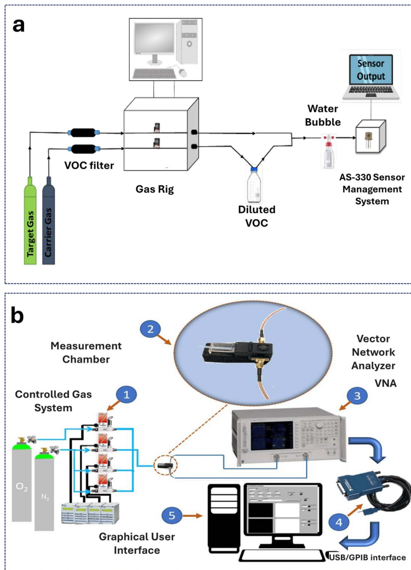
Fig. 10 VOC and oxygen gas sensor setups with detailed system components. (a) The diagram shows the target and carrier gas, VOC filter, gas rig, diluted VOC trap, water bubble for humidity, AS-330 sensor management system, and sensor output (reprinted with permission, 167 Copyright 2021, MDPI); schematic diagram of the oxygen gas sensor and (b) the set-up has five key parts: the controlled gas system, measuring chamber, vector network analyzer (VNA), USB/GPIB interface, and graphical user interface for oxygen monitoring (GPIB) (reprinted with permission, 166 Copyright 2020, MDPI).
