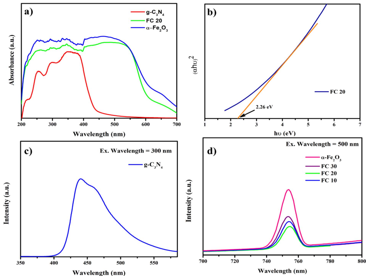
Fig. 6 UV-Vis DRS spectra of \alpha\text{-Fe}_2\text{O}_3 , g\text{-C}_3\text{N}_4 , and FC 20 (a), Tauc plot of FC 20 (b), and PL spectra of g\text{-C}_3\text{N}_4 (c), \alpha\text{-Fe}_2\text{O}_3 and heterostructures (d).
