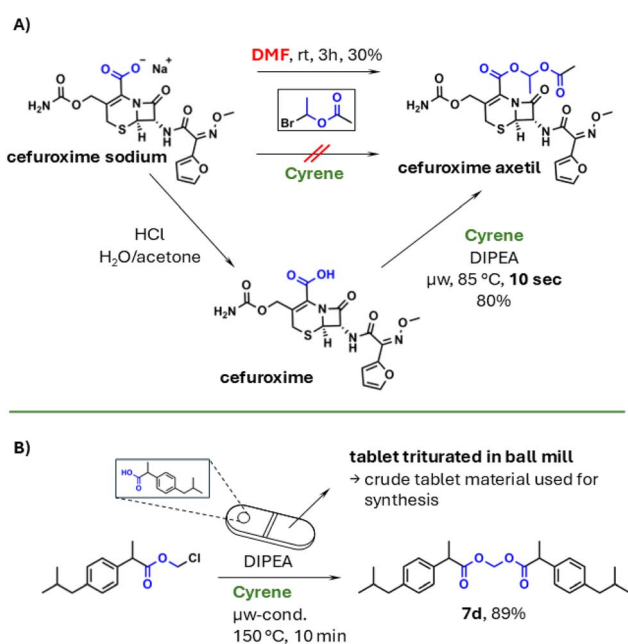
Fig. 5 (A) The synthesis of cefuroxime axetil from cefuroxime sodium failed due to insolubility of cefuroxime sodium in Cyrene. Despite complete solubility in DMF, the yield was unsatisfactory. Utilization of the free acid of cefuroxime for the synthesis leads to an ultra fast completion within seconds and very good yields. (B) The reaction of ibuprofen chloromethyl ester with ibuprofen from a crude matrix is not effected negatively by the excipients.
