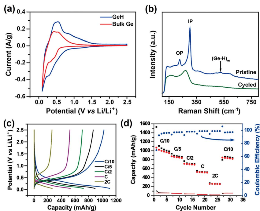
Fig. 6 (a) Comparison of CV diagrams for GeH and bulk Ge anode cycled between potentials of 2.5 and 0.1 V at a scan rate of 0.1 \text{mV s}^{-1} ; (b) ex situ Raman spectra for pristine (blue, top) and the Li-cycled (bottom, green) Ge anode, which shows indication for change in the structure associated in the delithiation driven amorphization of GeH sheet; (c) GCD profiles for GeH anode at different charge and discharge rates within a potential window of 0.1–2.5 V vs. \text{Li/Li}^+ ; (d) insertion and the extraction capacity retention for GeH anode plotted with a black square and red circle, respectively, and coulombic efficiency variation with respect to cycle number plotted with blue circles. The insertion and extraction capacity contributions from the carbon fiber/carbon black and poly(acrylic acid) binder are plotted as black and red lines, respectively. Reproduced with permission from ref. 41. Copyright (2017), the American Chemical Society.
