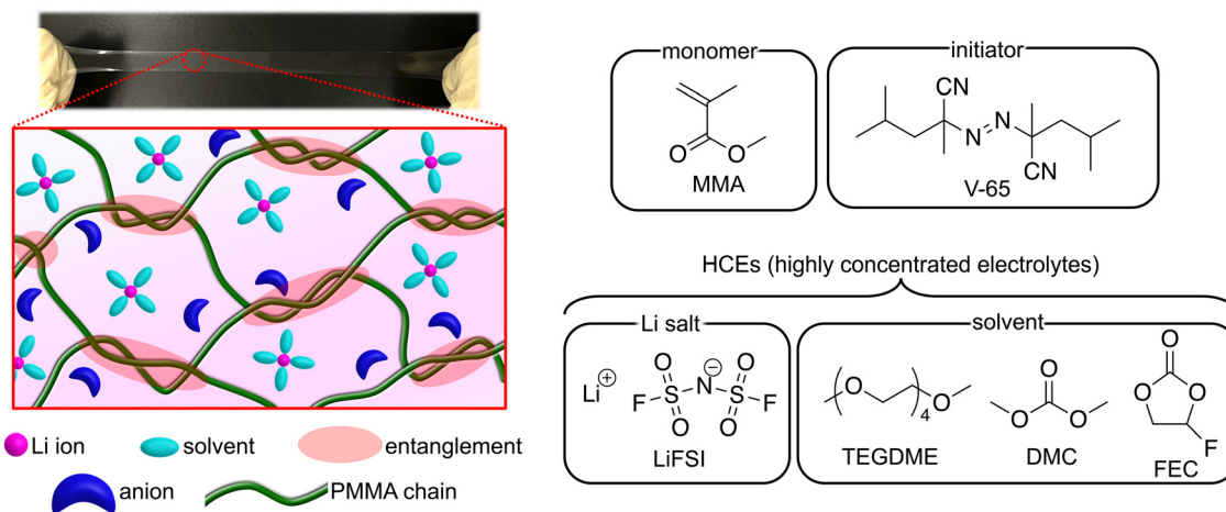
Fig. 1 Photograph and schematic of UHMW gel electrolytes containing HCEs, along with the chemical structures of the monomer, initiator, and HCEs.
