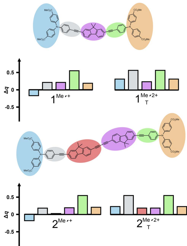
Fig. 5 Calculated electron density losses upon oxidation of model complexes 1^{\text{Me}\bullet+} and 2^{\text{Me}\bullet+} to their corresponding one- (left) and two-electron oxidized forms (triplet state), based on natural bond orbital (NBO) analysis. \Delta q refers to the charge difference of the respective molecular region of the radical monocations (left panels) and the respective dications in their triplet ground state (right panels) relative to the corresponding neutral state. The individual fragments are color-coded according to the graphical representation in the top panels.
