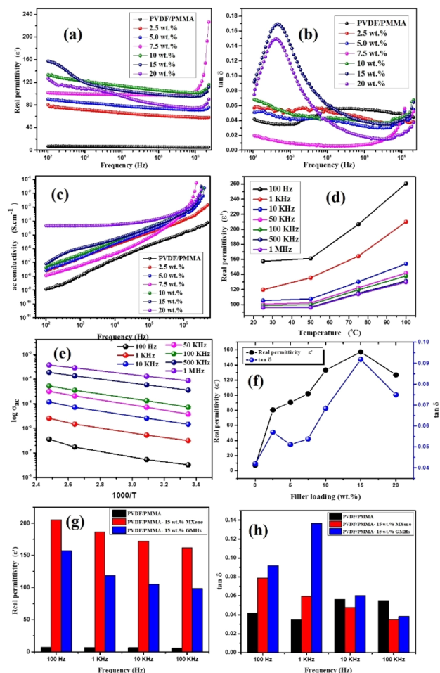
Fig. 5 Frequency dependence of (a) real permittivity, (b) \tan \delta and (c) ac conductivity, (d) temperature dependent \epsilon' and \tan \delta at different frequencies for 15 wt% HNCs, (e) plot of \ln(\sigma_{ac}) vs. 1000/T at different frequencies, (f) \epsilon' and \tan \delta with different wt% of GMH loading, (g and h) comparisons ( \epsilon' and \tan \delta ) of the PVDF/PMMA with 15 wt% MXene and 15 wt% GMH loading respectively.
