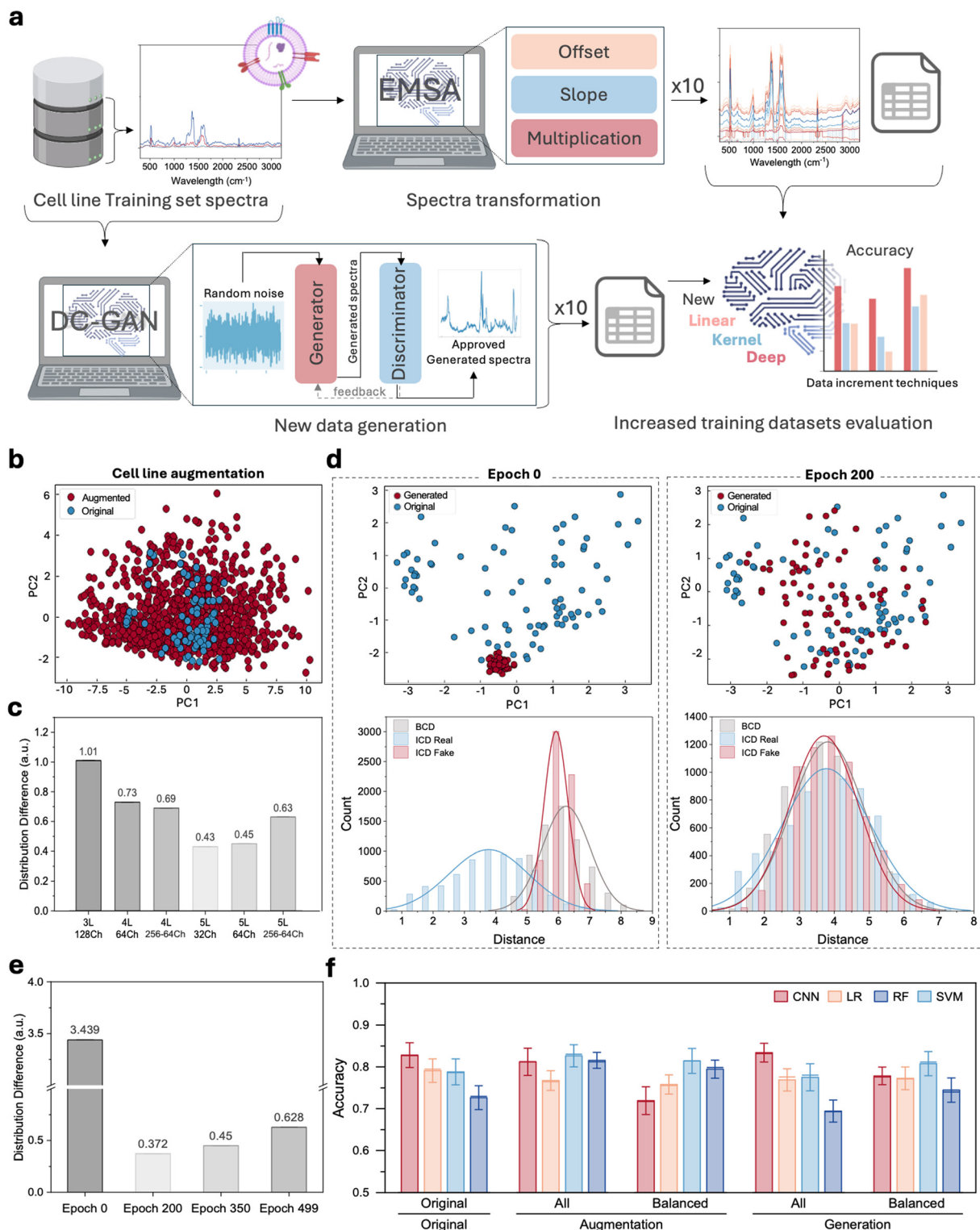
Fig. 3 Dataset augmentation via EMSA and DC-GAN. a) Task-i library is divided into training and test sets. The first is augmented 10-fold via EMSA which incurs in spectra transformation (offset, slope change, and multiplication). Simultaneously, the training set is used to train a DC-GAN model, taking Gaussian noise as input and modifying it to generate a spectrum similar to the original data. The newly increased datasets are evaluated with the models selected. b) EMSA augmented data compared to the original data (one cell line visualization). c) Different structures of the DC-GAN were tested and evaluated with the distribution difference (DD) metric. d) The selected structure is closely monitored through its training epochs, and the differences between the 0 epoch and the best-performing epoch (200) are visible in the PCAs and the histograms. The inter-class difference (ICD) real is a histogram of the original data, and the ICD fake is the one generated by the DC-GAN, the between-class distribution (BCD) showing the difference between them allows tracking the quality of the generated data. e) The different epochs of the selected structure are evaluated. f) The new larger training libraries were used to train our models and evaluated with the original Task-i test dataset in two conditions: a) all augmented observations and generated data are used and b) the new artificial data is used to balance the classes perfectly. The accuracy metric is calculated as previously described. Error bars represent \pm 1 standard deviation (SD) across 20 bootstrapping iterations of the test set, with replacement.
