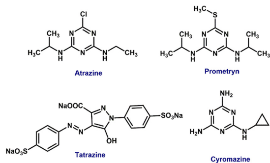
Fig. 27 Some common triazine pesticide derivatives.
