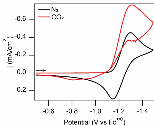
Fig. 3 Cyclic voltammograms of 1 mM [Fe(tpy)(Mebim-py)(NCCH 3 )](PF 6 ) 2 solution at an illuminated p-Si-CH 3 photoelectrode under a N 2 (black) and CO 2 atmosphere (red). Voltammograms recorded at 100 mV s -1 in 100 mM [NBu 4 ][PF 6 ] 95 : 5 CH 3 CN : H 2 O solution with a Pt mesh counter electrode (in a separate compartment), and an Ag/AgNO 3 reference electrode. Light source was a warm white light LED with an irradiance of 339 mW cm -2 . Arrow indicates starting point and scan direction.
