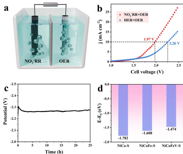
Fig. 5 (a) Two-electrode configuration schematic illustrating simultaneous OER (anode) and nitrate reduction ( \text{NO}_3\text{RR} , cathode) processes. (b) LSV curves of the electrolyzer under varied conditions: anolyte (1.0 M KOH) and catholyte (1.0 M KOH + 0.1 M \text{KNO}_3 ). (c) Chronopotentiometric test of the electrolyzer at 10 \text{ mA cm}^{-2} . (d) The statistics of d-band centers for NiCoFeV-S, NiCoFe-S, and NiCo-S.
