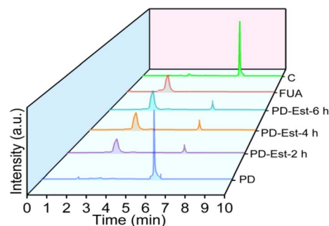
Fig. 2 RP-HPLC spectrum profile for PD, C, FUA, and Est-treated PD (50 \mu M each) after 2, 4, and 6 h in 1 \times PBS buffer solution.
